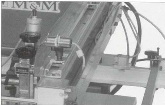
Stroke Length Sensors: Locate stroke length anywhere within the print area by adjustable slides.
