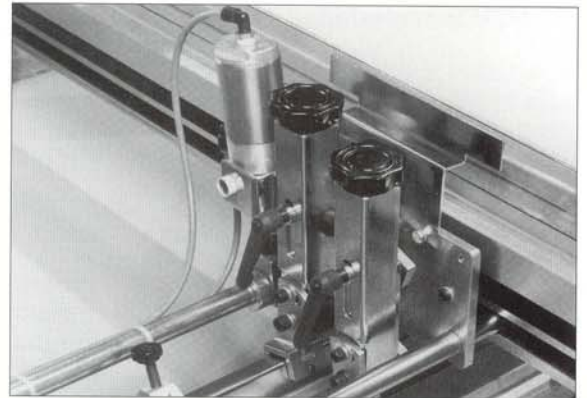
Squeegizer: Air controlled squeegee system automatically maintains uniform print pressure across the entire squeegee length and throughout the print stroke.
