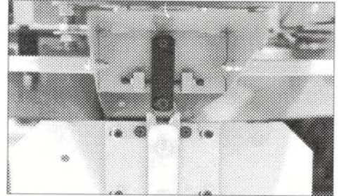
Pneumatic indexer locking fork provides \pm .001 " registration repeatability.
